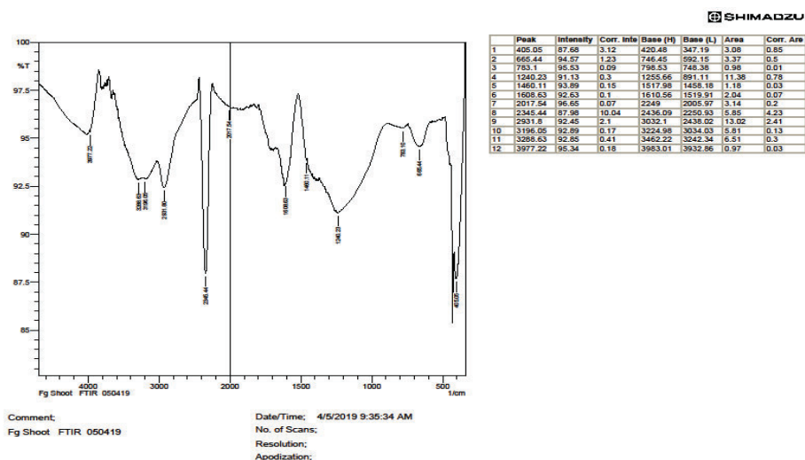
Fig. 7 FTIR spectrum of the soot sample of Calotropis gigantea
