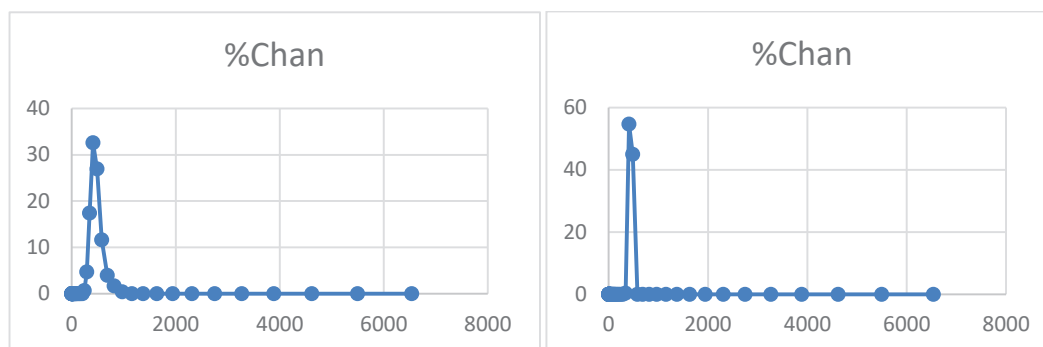
Fig. 6. Size range of soot sample of Calotropis gigantea and Parthenium hysterophorus (DLS)
