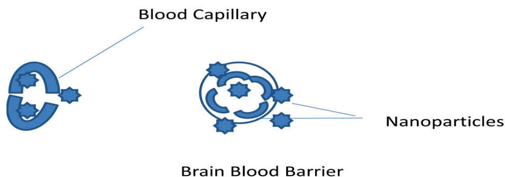
Fig. 2. Nanoparticles penetrating Blood Capillary and Blood Brain Barrier
