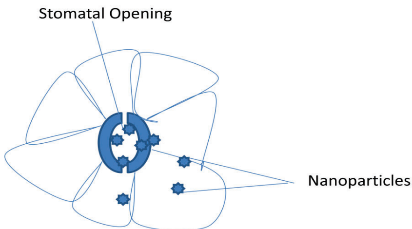
Fig. 4. Stomatal opening clogged with Nanoparticles
