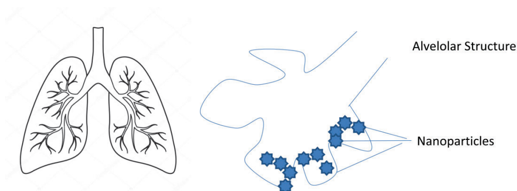
Fig. 1. Alveoli clogged with Nanoparticles.
