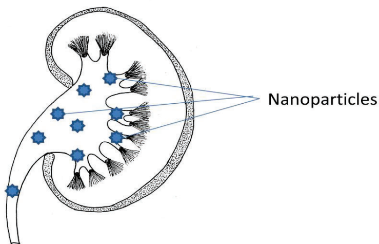
Fig. 3. Nanoparticles penetrating Kidney and affecting Renal system
