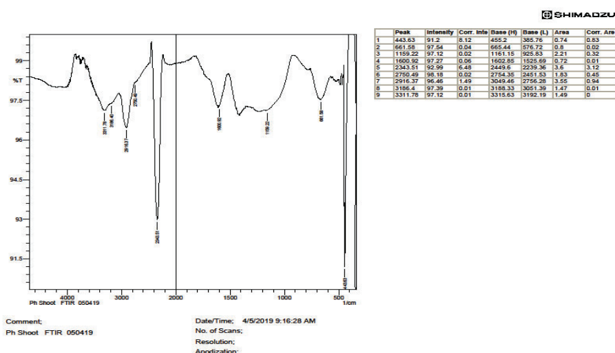
Fig. 8 FTIR spectrum of the soot sample of Parthenium hysterophorus
