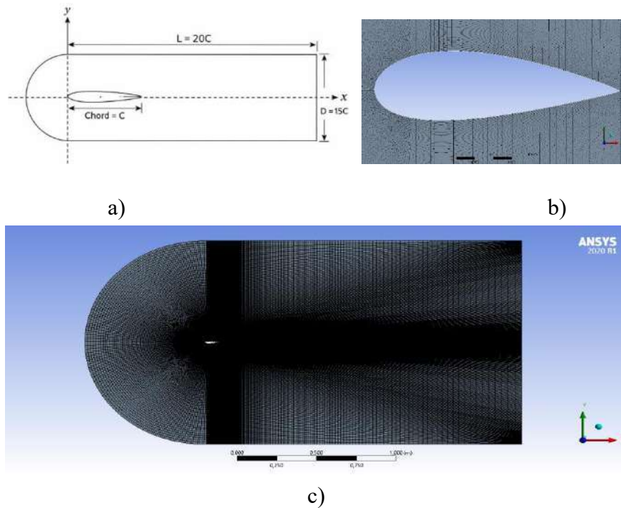
Figure 1. a) Boundary zone and conditions and, b) Mesh structure created in the analysis region
