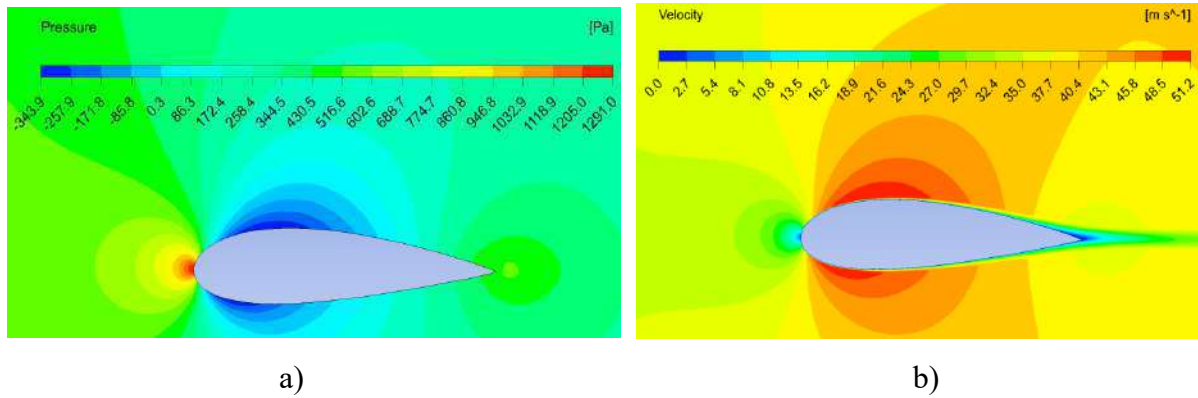
Figure 5. Aerodynamic contours at T = 15\text{ }^{\circ}\text{C} and Re = 100,000 with a) pressure and b) velocity
