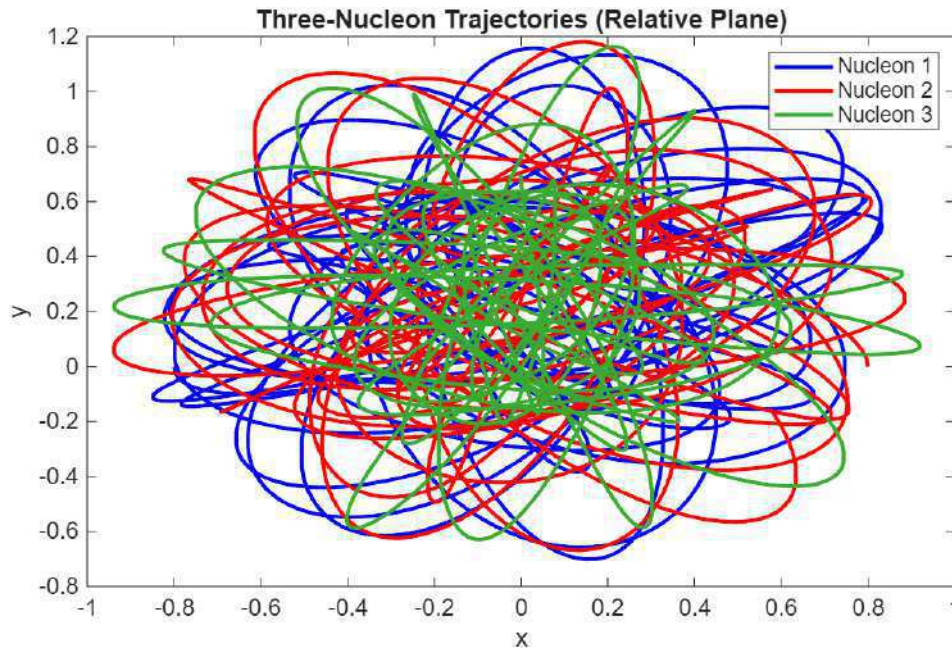
Figure 2. Trajectories of the three nucleons projected onto the relative coordinate plane using a symplectic integrator. The correlated motion demonstrates the stabilizing effect of the effective three-body interaction, preventing collapse and maintaining bounded dynamics over long integration times.
