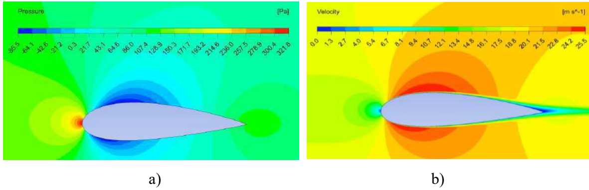
Figure 4. Aerodynamic contours at T = 15\text{ }^{\circ}\text{C} and Re=50,000 with a) pressure and b) velocity
