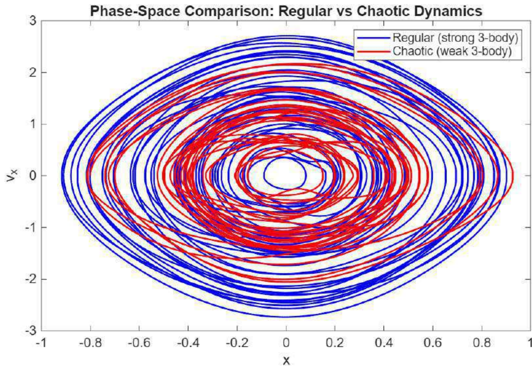
Figure 6. Phase-space projection ( x, v_x ) of a representative nucleon for two interaction regimes: strong three-body coupling (regular dynamics) and weak three-body coupling (chaotic dynamics). The regular regime exhibits confined quasi-periodic structures, whereas the weak-binding case leads to broader phase-space exploration, indicating enhanced sensitivity to initial conditions.
