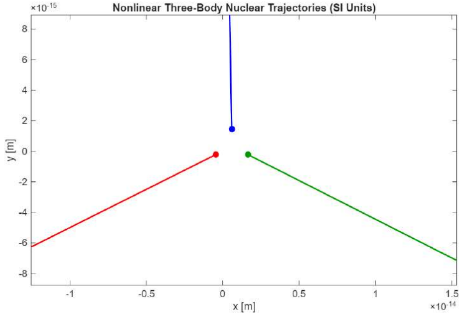
Figure 1. Trajectories of three nucleons projected onto the relative coordinate plane. The correlations induced by three-body forces stabilize the system and prevent collapse. Simulations without three-body interactions exhibit unphysical drift, highlighting the crucial role of three-body terms.
