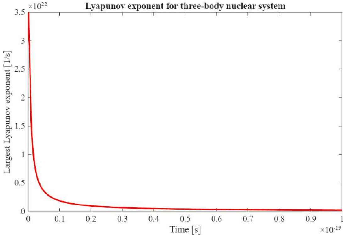
Figure 4. Time evolution of the largest Lyapunov exponent in the three-body nuclear system. Configurations with strong three-body binding display exponents near zero, indicating regular motion, while weaker binding leads to positive exponents, signaling chaotic behavior. All quantities are in SI units.
