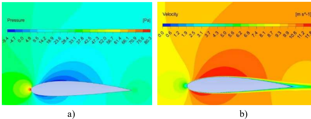
Figure 3. Aerodynamic analysis under Re = 50,000 conditions: a) Pressure distribution [Pa], b) Velocity magnitude distribution [m/s]
