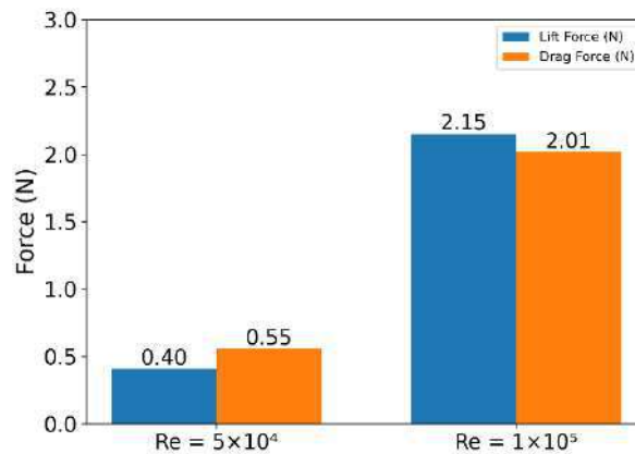
Figure 2. Lift and Drag Forces at T = -15\text{ }^{\circ}\text{C}
