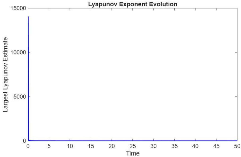
Figure 5. Time evolution of the estimated largest Lyapunov exponent for the three-body nuclear system. Positive values indicate exponential divergence of nearby trajectories, revealing sensitivity to initial conditions and the emergence of chaotic dynamics in weakly bound configurations.
