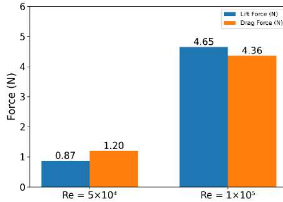
Figure 3. Lift and Drag Forces at T = 15\text{ }^{\circ}\text{C}
