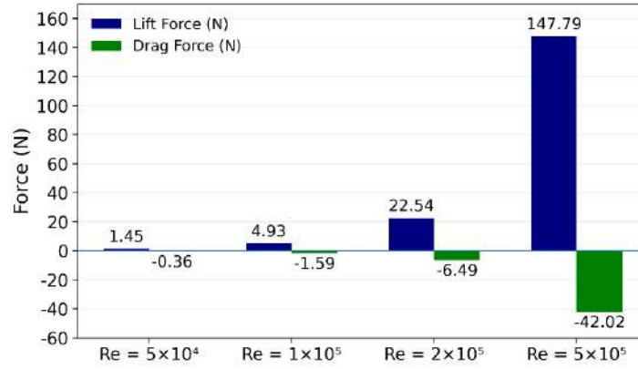
Figure 2. The lift and drag forces are presented for Reynolds numbers of 5 \times 10^4 , 1 \times 10^5 , 2 \times 10^5 and 5 \times 10^5
